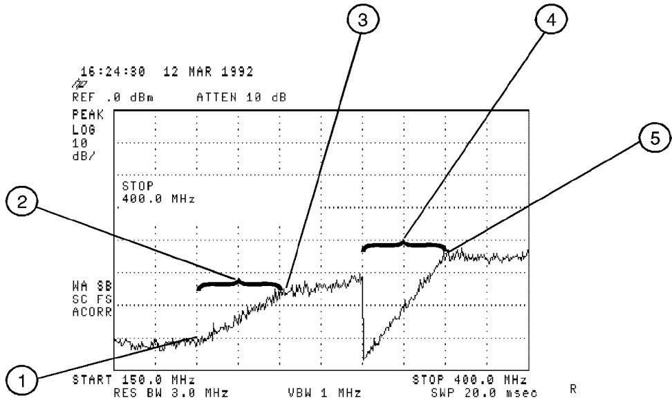
Figure 49 Amplitude-Correction Points
