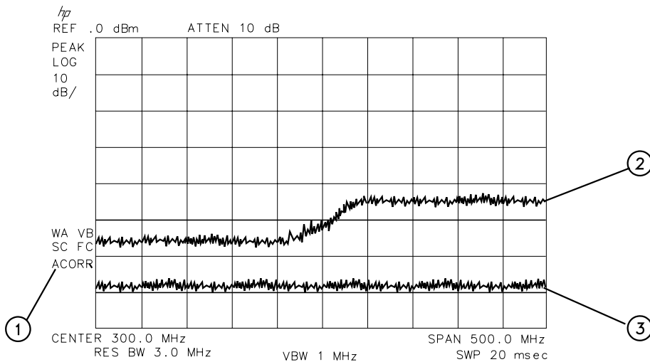
Figure 47 Amplitude-Correction Display
