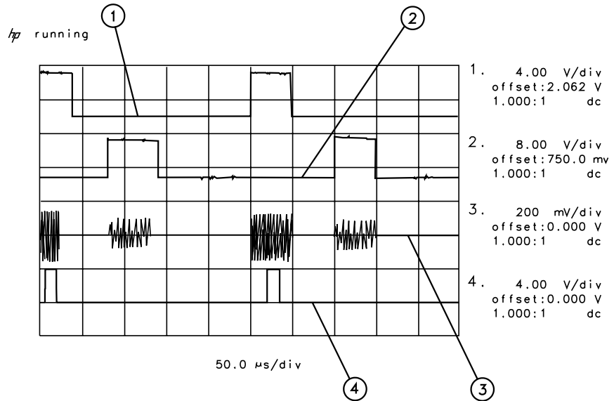
Figure 58 Setting the Gate Delay and Gate Length Using an Oscilloscope
